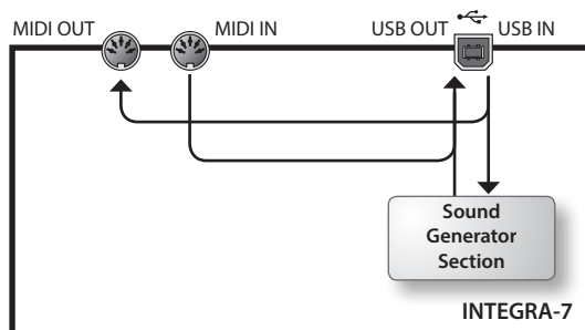
USB-MIDI Thru=ON
