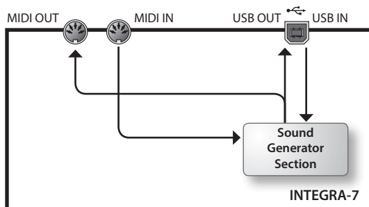
USB-MIDI Thru=OFF
